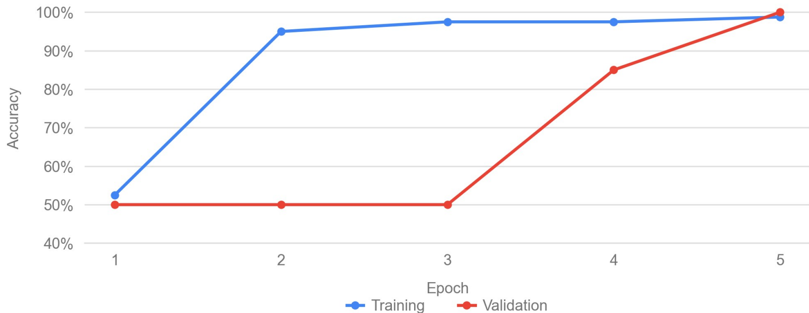
Accuracy per Epoch — Training vs Validation
